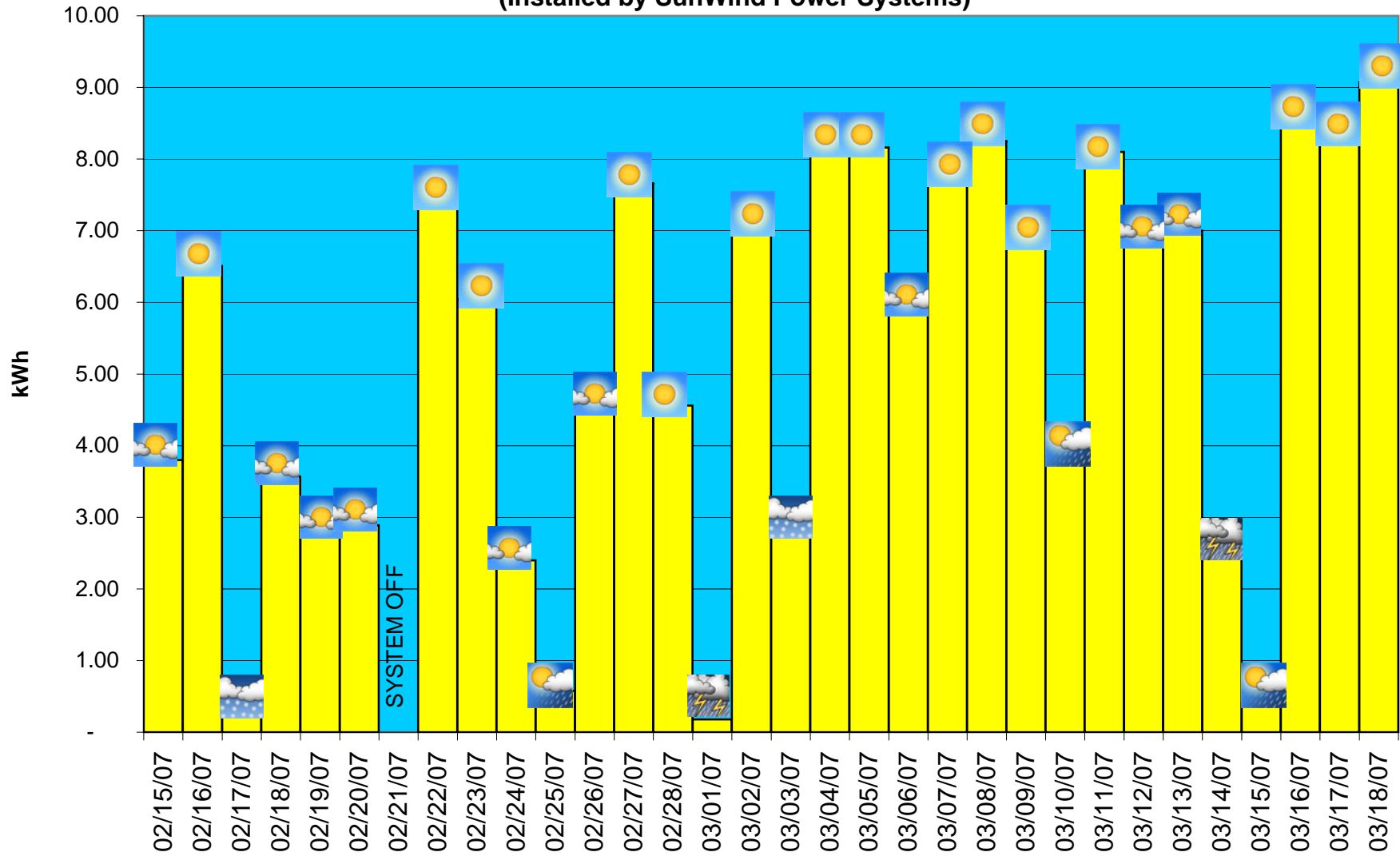
kWh Produced by Darst's PV System (Installed by SunWind Power Systems)
